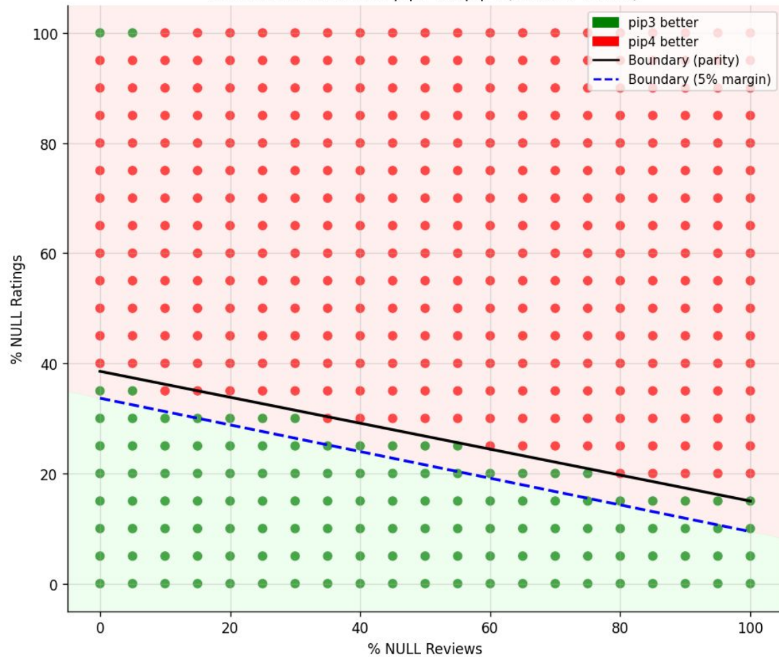
Decision boundaries: pip3 vs. pip4 (WMAPE-based)
